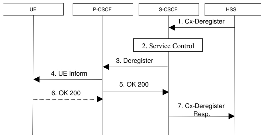
Figure 5.5: Network initiated application de-registration by HSS, administrative
