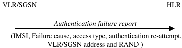
Figure 13: Reporting authentication failure from VLR/SGSN to HLR
