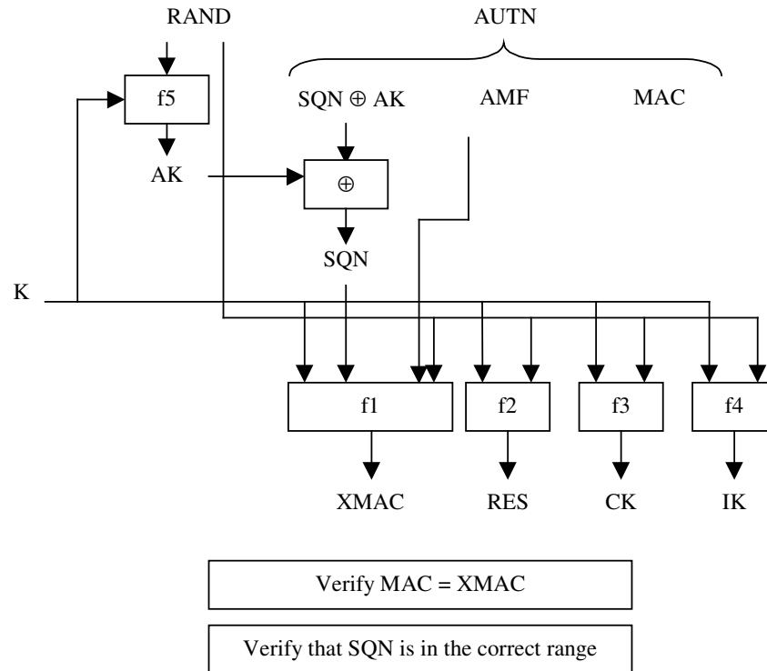
Figure 9: User authentication function in the USIM
