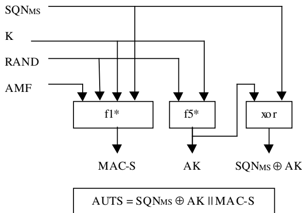
Figure 10: Construction of the parameter AUTS
