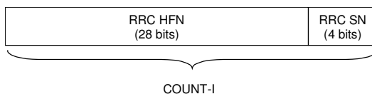
Figure 16a: The structure of COUNT-I
