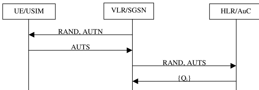
Figure 12: Resynchronisation mechanism
